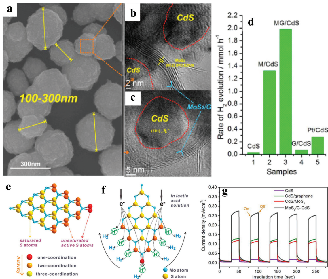
Fig. 2 (a) SEM image of CdS/MG nanocomposites after annealing at 573 K for 2 h under an Ar atmosphere, (b) and (c) HRTEM images of the CdS/MG nanocomposite. (d) Photocatalytic \text{H}_2 production activities of CdS, CdS/M, optimized CdS/MG, CdS/G, and Pt/CdS (0.5 wt%) in lactic acid solution, (e) schematic illustration of the microstructure of \text{MoS}_2 , and (f) its cocatalytic mechanism of \text{H}_2 generation. (g) Transient photocurrent responses of pristine CdS and its binary/ternary nanocomposite under simulated irradiation Copyright 2014, American Chemical Society. Reprinted from ref. 21 with permission.
