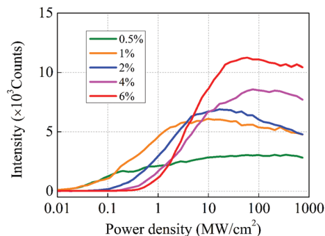
Fig. 2 Measured upconversion luminescence intensities of single UCNP s with different \text{Tm}^{3+} doping concentrations at different excitation power densities. Here, the intensity is the sum of the emission intensity for wavelengths in the range of 400–842 nm.
