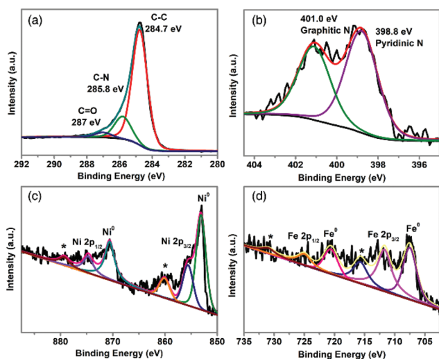
Fig. 3 High resolution XPS data for TA-NiFe@NCNT. (a) C 1s region, (b) N 1s region, (c) Ni 2p, and (d) Fe 2p.
