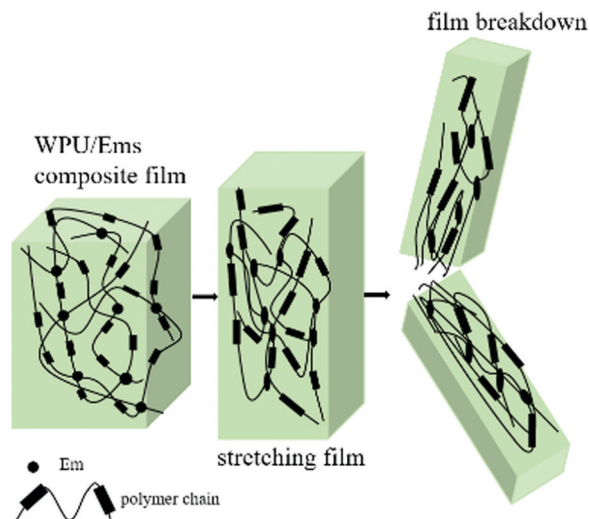
Fig. 10 Illustration of fracture mechanisms in the WPU/Ems composite film.
