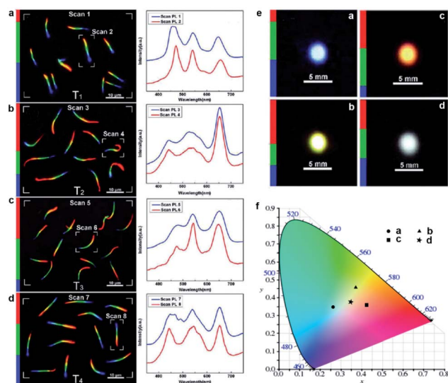
Fig. 6 White-light emission from composition-graded nanowires. (a–d) Real-color micrographs (left) and corresponding PL spectra (right) of dispersed \text{Zn}_x\text{Cd}_{1-x}\text{S}_x\text{Se}_{1-x} ( 0 \leq x, y \leq 1 ) nanowires from four tri-color samples (samples T1–T4), under 355 nm laser illumination. (e) Large area real-color photographs of the four samples under the illumination of a UV light beam. (f) CIE chromaticity diagram with the chromatic coordinates of the four tricolor samples calculated using the PL spectra shown on the right side of panels (a–d), respectively. Reproduced with permission. 12 Copyright 2011, American Chemical Society.
