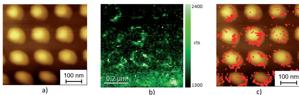
Fig. 6 (a) AFM topography image of the Au nanodisk array with CdSe NCs. (b) TERS intensity image of LO phonon mode from CdSe NCs, obtained simultaneously with the AFM image shown in (a). (c) Superposition of the AFM image and TERS intensity from the same sample area indicating that the strong TERS signal originates predominantly from the Au nanodisk edges. (c) is created by overlaying the background subtracted TERS map (b) on top of the AFM topography (a).
