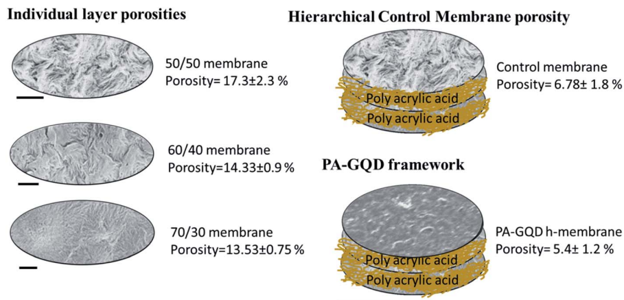
Fig. 15 Role of individual layers and their arrangement in selectively remediating dye pollutants and salt ions. The scale bar indicated is 2 \mu m.
