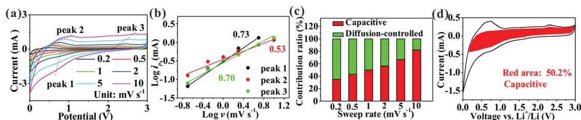
Fig. 6 (a) CV curves at different scanning rates; (b) the line relationship of \log(i_p) vs. \log(\nu) at peaks 1–3 marked in (a); (c) the percentages of the pseudocapacitive contribution at different scanning rates; and (d) the detailed pseudocapacitive contribution at a scanning rate of 1 mV s -1 of SnO 2 @TiO 2 /C.
