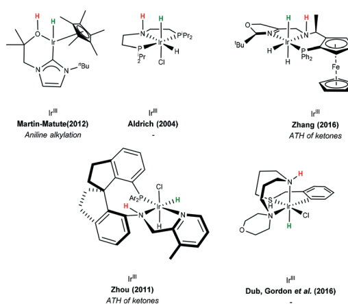
Scheme 39 Examples of metal-ligand bifunctional catalysts.
