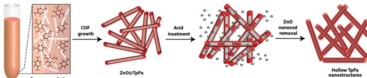
Fig. 8 Scheme of the formation of hollow COFs via a templating strategy. Reproduced with permission from ref. 137. Copyright 2015, Royal Society of Chemistry.
