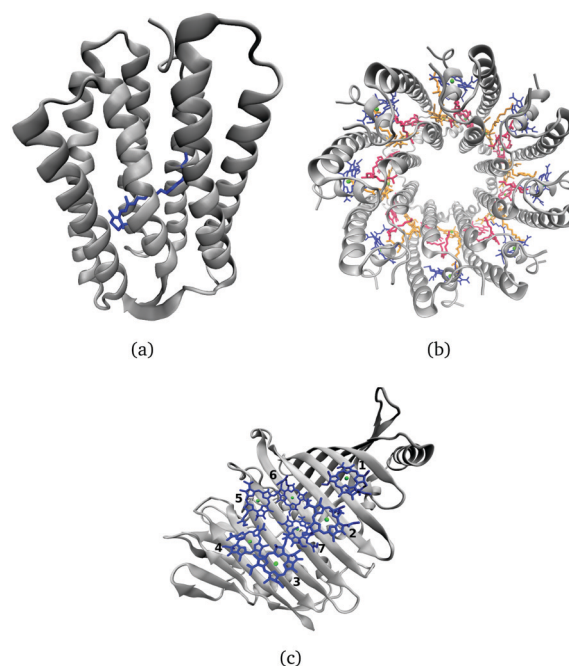
Fig. 2 (a) Side view of a rhodopsin model, here bR, with retinal in blue. (b) Top view of the LH2 complex from Rs. molischianum with the BChla chromophores of the B800 ring colored in blue and those belonging to the B850 ring in red and orange. (c) FMO monomer with seven BChla chromophores.
