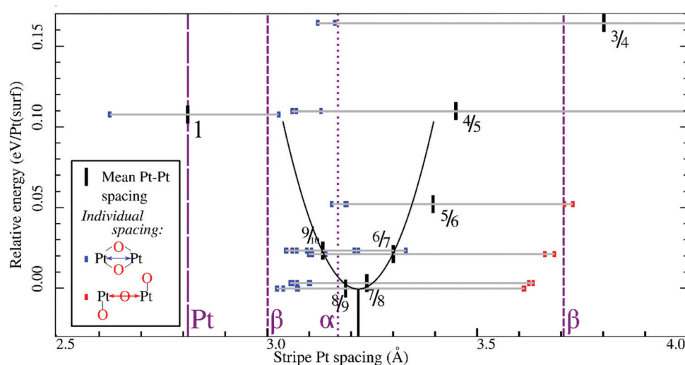
Fig. 4 Relative stripe formation energies (per surface platinum atom, without vibrational contribution) versus individual Pt–Pt distances (in the stripe) and mean spacings, including a quadratic fit of mean spacings near the energy minimum (marked by a descender from the apex of the parabola) and bulk Pt–Pt spacings for Pt, \alpha -PtO 2 and \beta -PtO 2 ; legend in inset.
