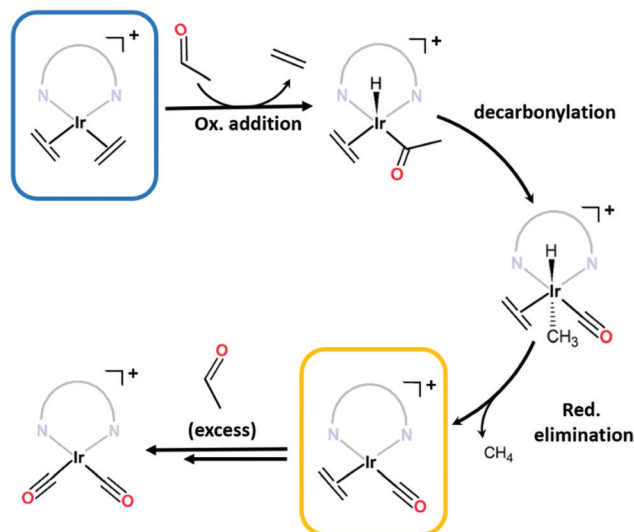
Fig. 2 The proposed mechanism via which mono- and dicarbonyl complexes are generated from decarbonylation of acetaldehyde. The target bis(ethylene) complex 1 -IrCl(ETH), and the 1 -IrCl(ETH/CO) by product that is also observed, are shown in the blue and yellow boxes. Acetaldehyde can be formed by dehydrogenation of ethanol.
