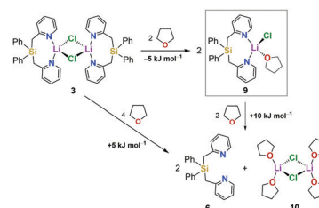
Scheme 2 Calculated reaction enthalpies ( \Delta H ) for the proposed dissociation of dimer 3 into a monomeric LiCl complex ( 9 ) and for the unlikely dissociation into the free ligand 6 and a dissolved LiCl·THF complex ( 10 ) in THF [B3LYP/6-31+G(d)] (PCM calculations; solvent: THF).
