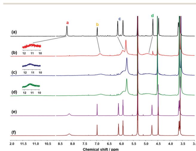
Fig. 3 ^1\text{H} NMR spectra of (a) 1 (5 mM) and 1 after extraction with (b) LiCl(aq), (c) LiCl(s), (d) a mixture of LiCl(s), NaCl(s) and KCl(s), (e) excess NaCl(s), and (f) excess KCl(s).
