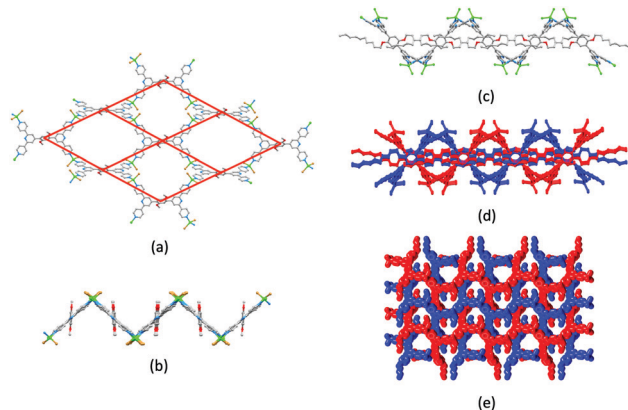
Fig. 5 (a) Part of the (4,4)-net in [\text{Zn}_2\text{Br}_4(\mathbf{1})]_n (CSD refcode ZUGVII, H atoms omitted); ligand 1 is a 4-connecting node. (b) The same net viewed through the mean plane through the ligand nodes showing the orientation of the MeO groups above and below the plane. (c) Part of one (4,4)-net in [\text{Zn}_2\text{Cl}_4(\mathbf{6})]_n (CSD refcode DAQMIU, H atoms omitted) and (d) and (e) two views of 2D \rightarrow 2D parallel interpenetrated nets in [\text{Zn}_2\text{Cl}_4(\mathbf{6})]_n .
