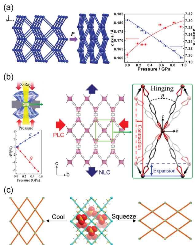
Fig. 16 Scheme of the wine-rack structural changes under hydrostatic pressure that exhibit NLC. (a) [NH 4 ][Zn(HCOO) 3 ]. (b) InH(BDC) 2 . (c) [Ag(ethylenediamine)]NO 3 . Partly taken from ref. 111, 113, and 116 with permission.
