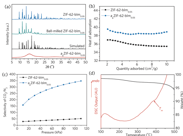
Fig. 2 (a) XRD spectra of ZIF-62-bIm 0.05 crystals and a g ZIF-62-bIm 0.05 glass, (b) heat of CO 2 adsorption for ZIF-62-bIm 0.05 and a g ZIF-62-bIm 0.05 , (c) IAST adsorption selectivity of ZIF-62-bIm 0.05 crystal and a g ZIF-62-bIm 0.05 for 50/50 CO 2 /N 2 mixture at 303 K, (d) thermogravimetric (TG) and differential scanning calorimetry (DSC) analysis for (ZIF-62) 0.2 (6FDA-DAM) 0.8 composite.
