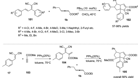
Scheme 32 Phosphine-catalysed sequential (2+3) and (3+2) annulation reactions of \gamma -substituted allenones with conjugated dienes.
