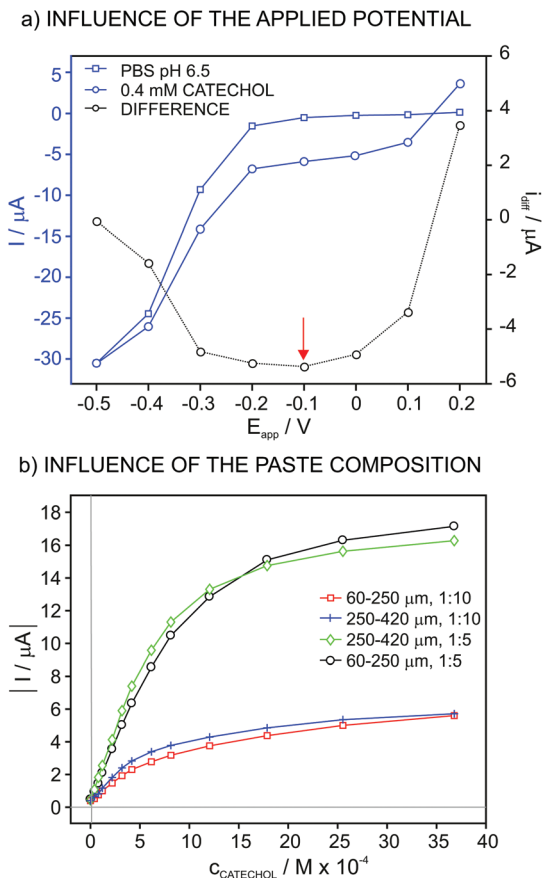
Fig. 1 Influence of (a) the applied potential and (b) paste composition and particle size on the recorded current.
