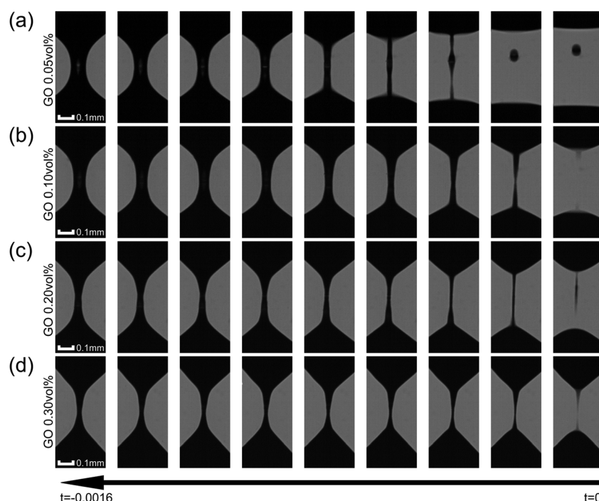
Fig. 3 Images of capillary thinning and breakup of the filament for GO suspensions for concentrations between 0.05 vol% and 0.3 vol% tested in the CaBER. The time interval between consecutive images is 0.165 ms. The images show the different behaviours near breakup for different concentrations. At 0.05 vol% GO (a) the filament exhibits a Newtonian-like behaviour. As concentration increases up to 0.4 vol% the filament does not form a straight-walled column immediately prior to breakup and conical tapering becomes evident (b–d).
