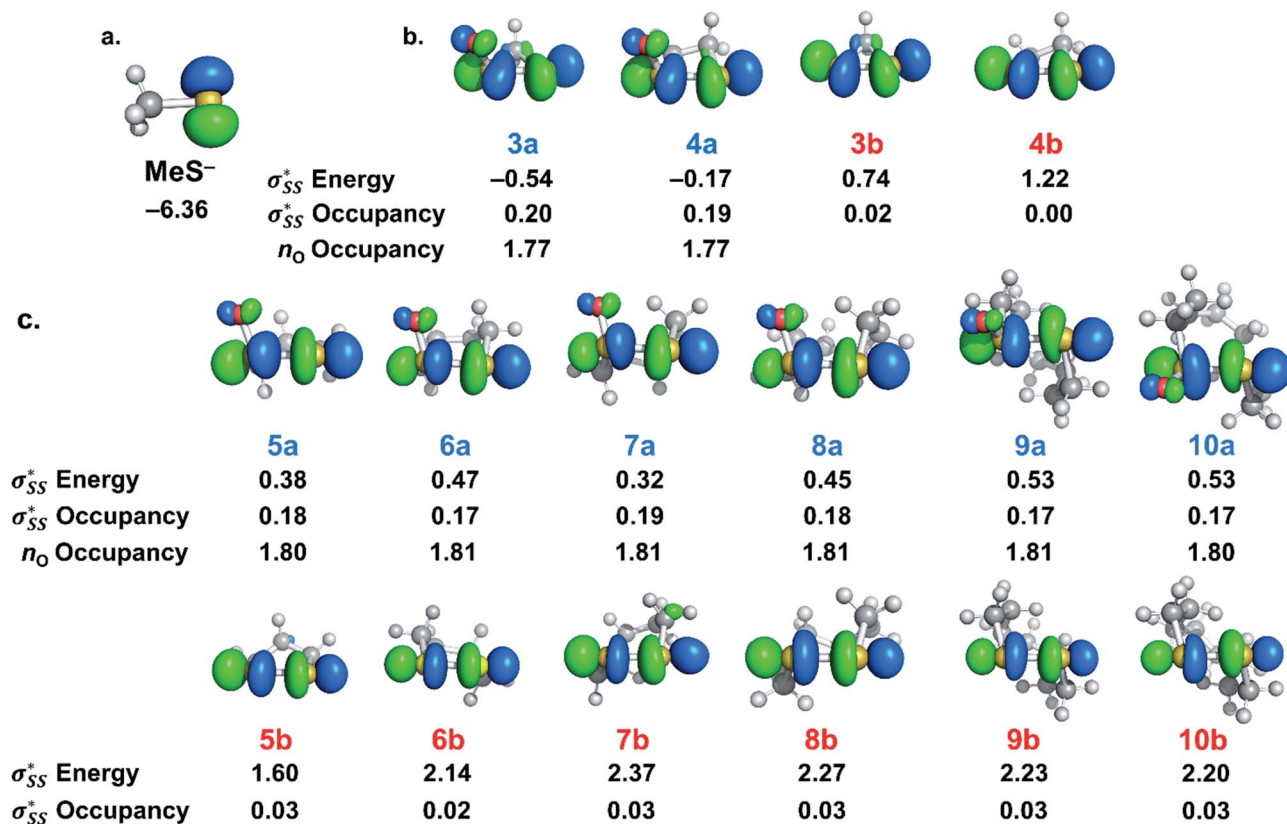
Fig. 7 (a) Visual representation of MeS^- HOMO and corresponding orbital energy. (b) Visual representation of \sigma_{SS}^* orbitals of (3–4) a and (3–4) b and the corresponding orbital energies and occupancies. (c.) Visual representation of \sigma_{SS}^* orbitals of (5–10) a and (5–10) b and the corresponding orbital energies and occupancies. Computed M06-2X/6-311++G(d,p) IEF-PMCH 2 O. Energies are reported in eV.
