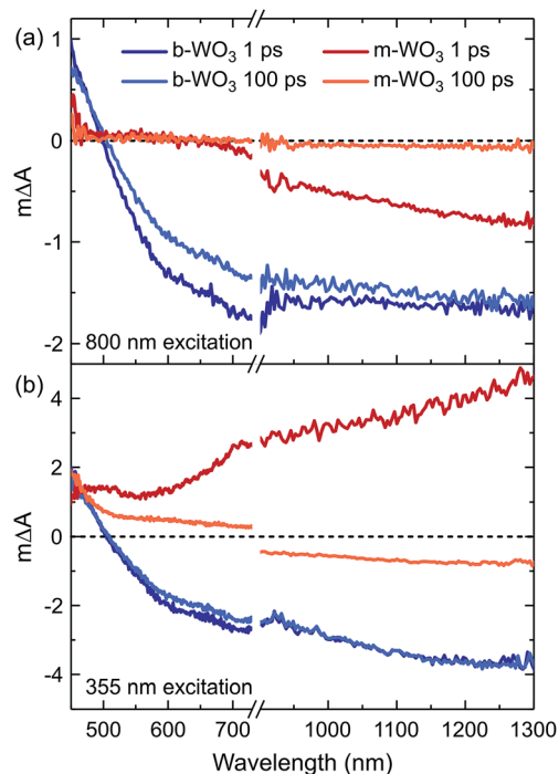
Fig. 4 Transient absorption spectra of m-WO 3 and b-WO 3 for excitation wavelengths of (a) 800 nm and (b) 355 nm. For each sample and excitation wavelength, spectra probed at 1 ps and 100 ps after excitation are shown. All spectra were acquired at an excitation intensity of 0.26 mJ cm -2 under argon atmosphere.
