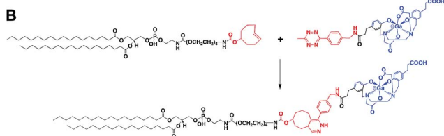
Fig. 4 (A) Radio-HPLC chromatograms of (top) [^{68}\text{Ga}]\text{Ga-HBED-CC-tetrazine} precursor and (bottom) reaction between 4 and 5, after 15 min at 60 ^{\circ}\text{C} . (B) Scheme of the reaction between TCO-modified PE (4) and [^{68}\text{Ga}]\text{Ga-HBED-CC-tetrazine} (5).
