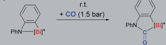
Scheme 1 Examples of well-defined compounds of heavy p-block elements that show unusual reactivity patterns towards small molecules. Aryl = \text{C}_6\text{H}_3\text{--}2,6(\text{C}_6\text{H}_3\text{--}2,6\text{-iPr}_2)_2 .
