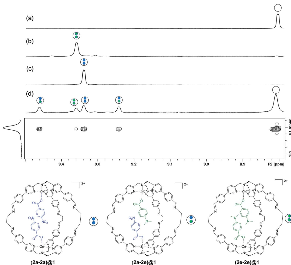
Fig. 3 Partial 500 MHz 1 H NMR spectra showing the signals due to the cage pyridine α protons (301 K, CD 3 CN) for (a) cage 1 (b) (2e-2e)@1 (c) (2a-2a)@1 and (d) 1 H ROESY experiment for the competition experiment between guest 2a and 2e ([ 1 ] = 1.0 mM, [ 2a ] = [ 2e ] = 0.1 mM). Counterions are perchlorate for the cage and triethyl ammonium for the guest and they are omitted for clarity.
