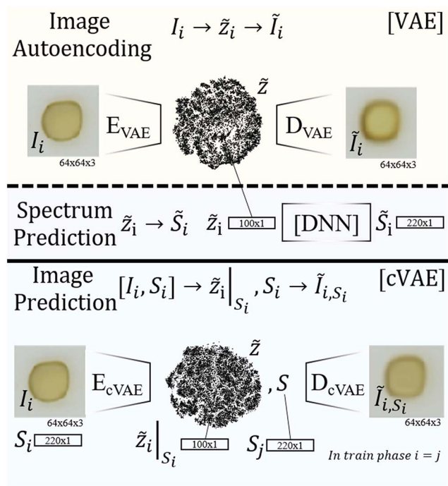
Fig. 1 Schematic visualization of the 3 types of learning models for optical properties of materials. The first algorithm (top) illustrates the variational autoencoder (VAE) that autoencodes images I_i from I_i via a latent space representation Z_i . The encoder performing the mapping I_i to Z_i is called E_{VAE} , the decoder performing the mapping from Z_i to I_i is called D_{VAE} . The second model employs the latent space of the VAE but decodes Z_i into an absorption spectrum S_i (instead of an image) using a deep neural net (DNN), producing an image to spectrum prediction model. The cVAE reconstructs images I_i from images I_i and spectra S_i such that the latent space vector Z_i encodes image and spectral information, which is decoded in conjunction with a specific absorption spectrum S_i to yield an image that is predicted to exhibit the specified absorption properties.
