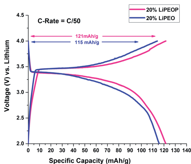
Fig. 6 Charge–discharge cycles showing the effect of addition of PDMS in 20% PEO electrolyte on the 2 nd cycle of charge–discharge of LiFePO 4 half cells at 60 °C.
