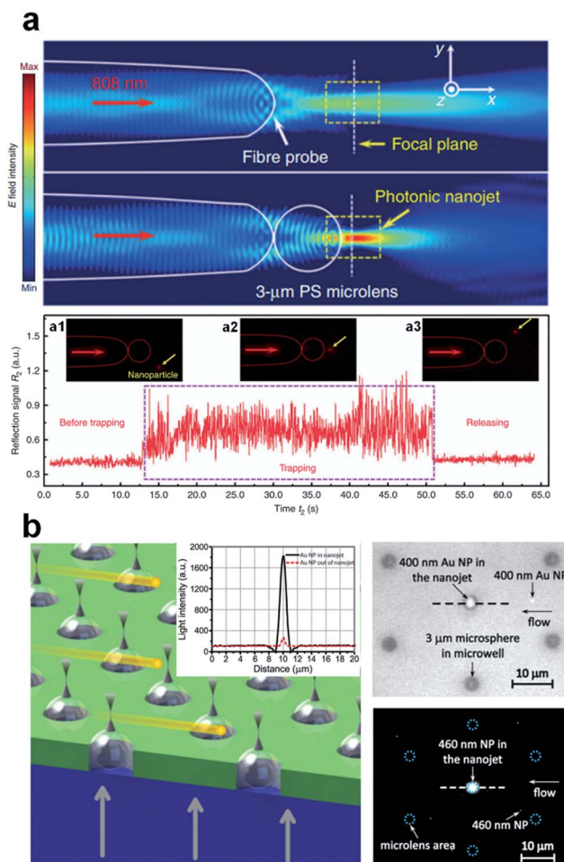
Fig. 12 (a) The real-time trace of the reflected 808 nm signal in the trapping process of an 85 nm fluorescent nanoparticle, and optical images showing the dynamic trapping of nanoparticles and plasmid DNA molecules. The insets in the bottom sub-figure of (a) show the fluorescent images (a1) before trapping, (a2) during trapping, and (a3) in the release. Reproduced with permission from ref. 296. Copyright 2016, Nature Publishing Group. (b) Schematic illustration of the optical detection of nanoparticles, and optical images showing the detected nanoparticles by the PNJ array. Reproduced with permission from ref. 298. Copyright 2015, American Chemical Society.
