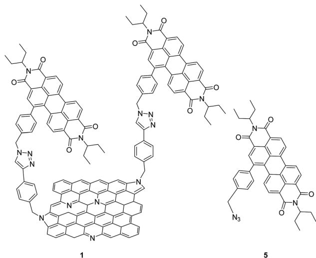
Fig. 1 Structures of the N-doped graphene–perylene-3,4,9,10-tetracarboxylic diimide hybrid, 1 , and control PDI 5 , investigated in the present study.
