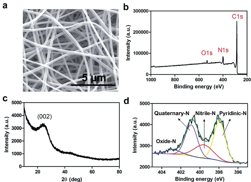
Fig. 1 SEM image of nCNFs produced at 800 ^{\circ}\text{C} (a), Survey XPS spectrum (b), XRD spectrum (c) and deconvoluted XPS spectrum (d) of N1s of nCNFs.
