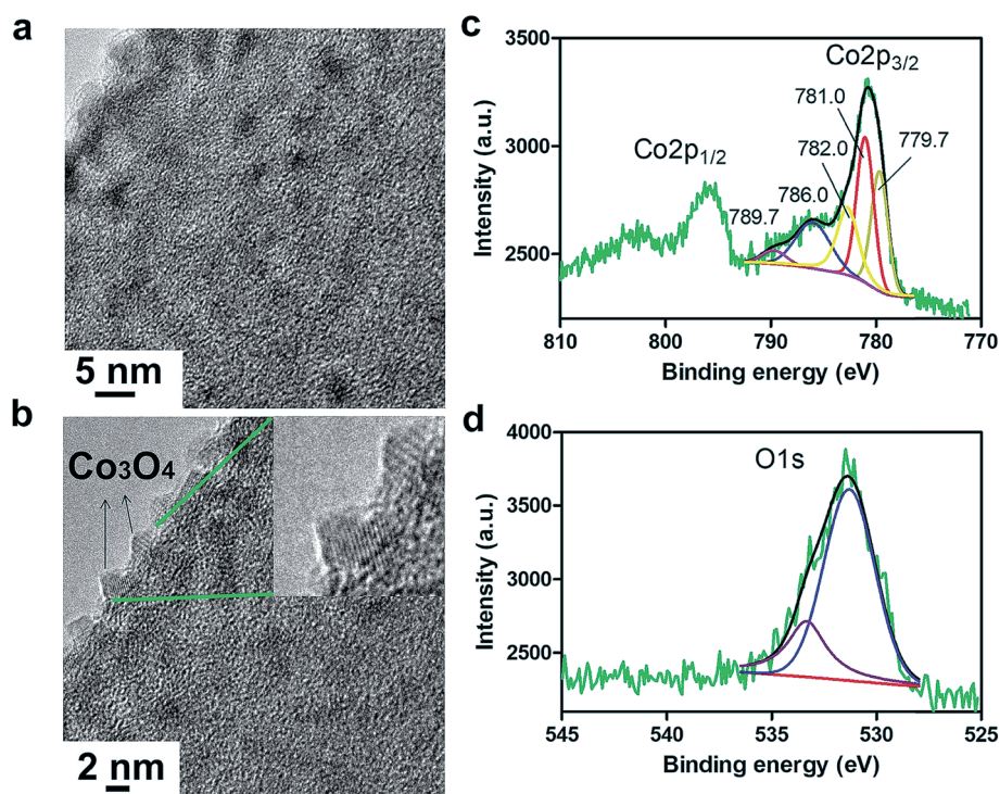
Fig. 2 TEM (a) and HRTEM (b) images of Co100@nCNFs. The inset shows the crystalline spinel structure of \text{Co}_3\text{O}_4 nanoparticles. Deconvoluted XPS spectra of Co2p (c) and O1s (d) for Co100@nCNFs.
