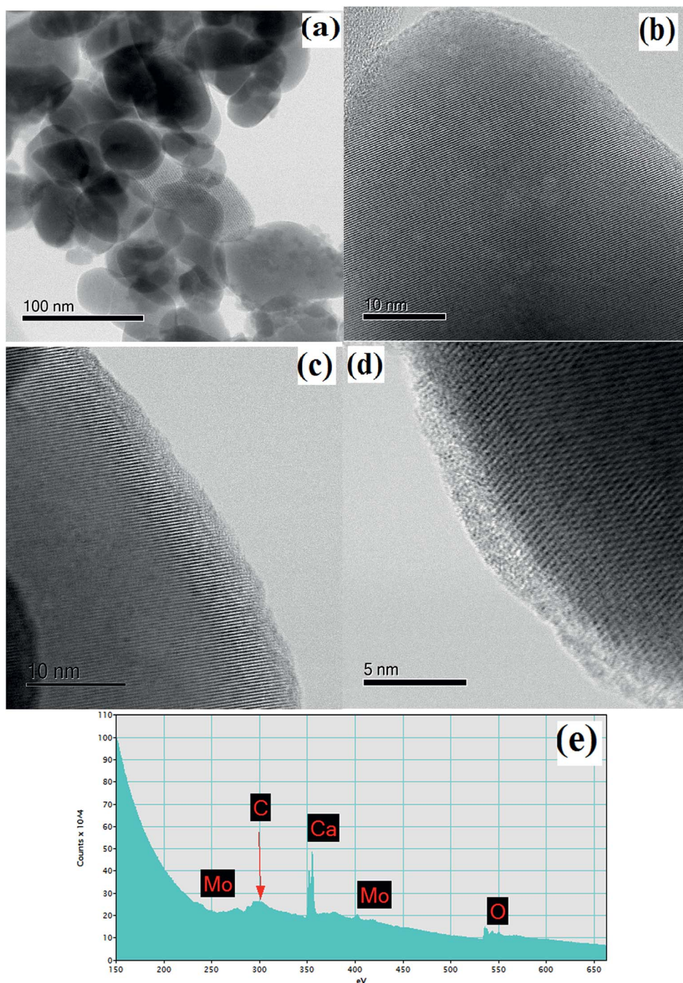
Fig. 8 STEM images/spectra of \text{CaMoO}_4 synthesized at 300^\circ\text{C} showing: (a) a bright field image of the rounded particles with small pores between them; (b) details of a particle showing a dispersion of fine scale spherical porosity (bright regions within the crystal) 2–5 nm in diameter; (c) and (d) atomic resolution bright field images showing the presence of (c) a thin (<2 nm) and (d) thicker (2–3 nm) surface amorphous layer on the otherwise crystalline particles and the amorphous layer was identified as being carbon; (e) EELS spectrum of (d) showing a distinct carbon peak.
