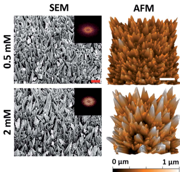
Fig. 3 Native surface data for the \text{Pb}^+ concentration series: column (1) SEM (45° tilted) and column (2) AFM images of the gold nanospike surfaces for 0.5 and 2 mM \text{Pb}(\text{CH}_3\text{COO})_2 . The 2D-FFT data is shown for the top-down SEM images (see Fig. S5†). The red and white scale bars are 200 nm and 1 \mu\text{m} , respectively.
