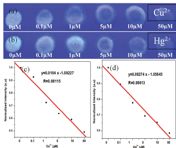
Fig. 9 Digital photograph, under 365 nm UV lamp, of NCDs in circular reaction pots on interaction with different concentrations (0.1 \mu\text{M} to 50 \mu\text{M} ) of (a) \text{Cu}^{2+} and (b) \text{Hg}^{2+} . Fluorescence intensity versus metal ion concentration plot (c) corresponding to (a) and (d) corresponding to (b) (fluorescence intensity of the filter paper loaded NCDs with an increase in concentration of \text{Cu}^{2+} or \text{Hg}^{2+} ions, analysed with ImageJ software).
