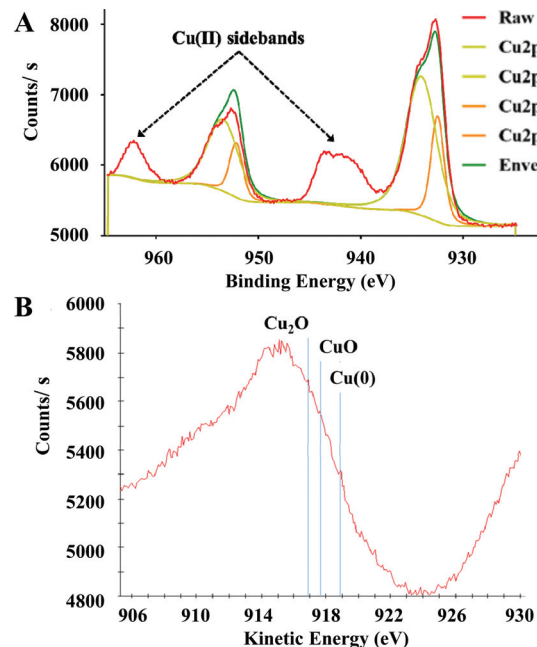
Fig. 6 (A) X-ray photoelectron spectroscopy (XPS) data of recovered Cu8/MgAlO x -HP (with peak fitting) and (B) Auger LMM spectra of recovered Cu8/MgAlO x -HP.
