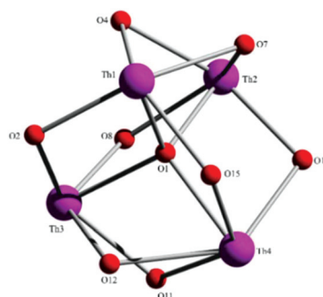
Fig. 2 The \{\text{Th}_4^{\text{IV}}(\mu_4\text{-O})(\mu\text{-OR})_8\} core of molecules 1 and 2 . O1 is the \mu_4\text{-O}^{2-} group in 1 , O4 and O12 are the bridging oxygen atoms of the iminiumphenolate parts of the \text{LH}^- in 1 ligands, while the remaining oxygen atoms belong to the \text{L}^{2-} groups.
