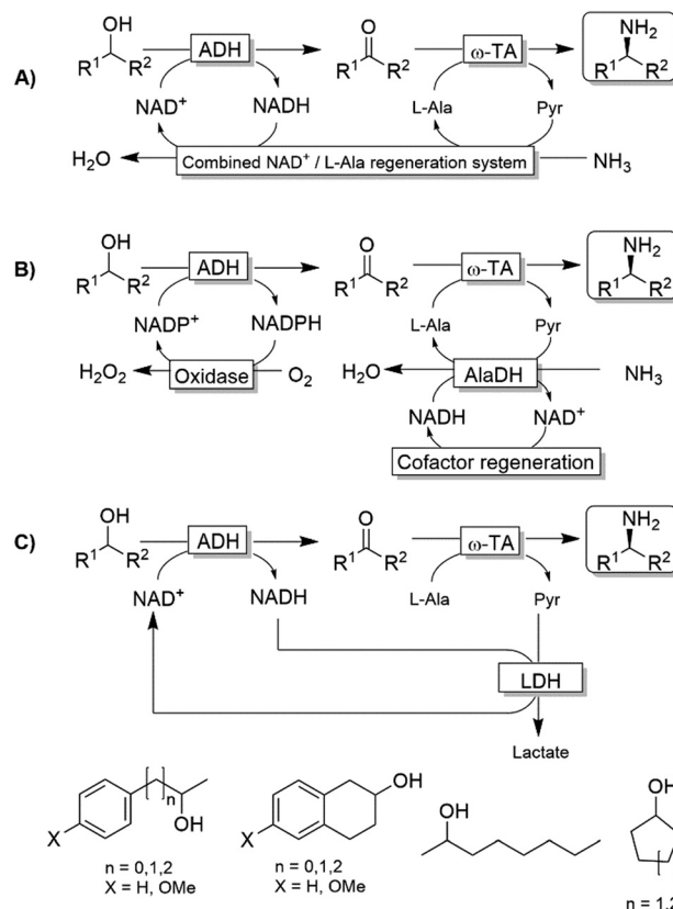
Scheme 23 Redox-neutral systems emulating an aza-Mitsunobu reaction comprising ADH-catalysed oxidation of an alcohol followed by the ω-TA-catalysed reductive amination. A) The combined \text{NAD}^+ /L-Ala regeneration system comprises L-AlaDH-catalysed reductive amination of pyruvic acid. L-AlaDH: L-alanine dehydrogenase (EC 1.4.1.1). B) Variation of the system comprising orthogonal oxidation and amination steps. C) Variation of the system with pyruvate-removal coupled with \text{NAD}^+ -regeneration. Although only system C generates a stoichiometric amount of lactate as waste, all the systems require a supra-stoichiometric amount of alanine as sacrificial amine donor.
