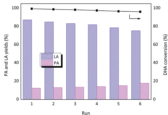
Fig. 8 Results of the reusability study (conditions: [\text{DHA}]_0 = 0.2 \text{ M} , \text{SnO}_2/\text{Nb}_2\text{O}_5 -3.07 = 50 mg, 140 °C, 1 h).
