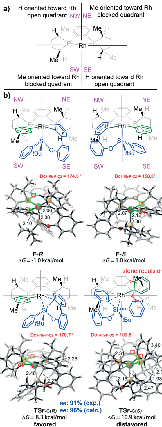
Fig. 5 (a) Quadrant analysis of the chiral environment created by the ( S,S )-Me-Duphos ligand. (b) Optimized structures of F-R , F-S , TS_{F-C(R)} and TS_{F-C(S)} . Distances are given in angstroms and angles in degrees.
