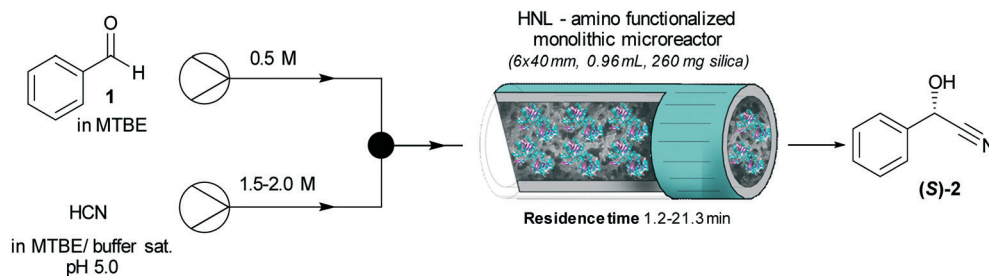
Scheme 2 Synthesis of (S)-mandelonitrile ((S)-2) in buffer saturated MTBE (citrate/phosphate (pH 5.0, 50 mM)) continuous flow reaction system with HNL immobilized on amino functionalized (and glutaraldehyde activated) siliceous monolithic microreactor.
