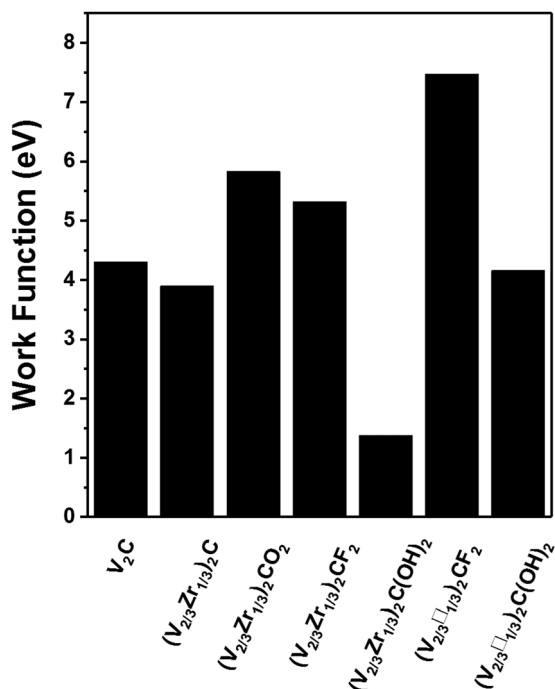
Fig. 5 Work functions of V_2C , pristine (V_{2/3}Zr_{1/3})_2C , bimetallic (V_{2/3}Zr_{1/3})_2CO_2 and vacancy-ordered (V_{2/3}\square_{1/3})_2C MXenes.
