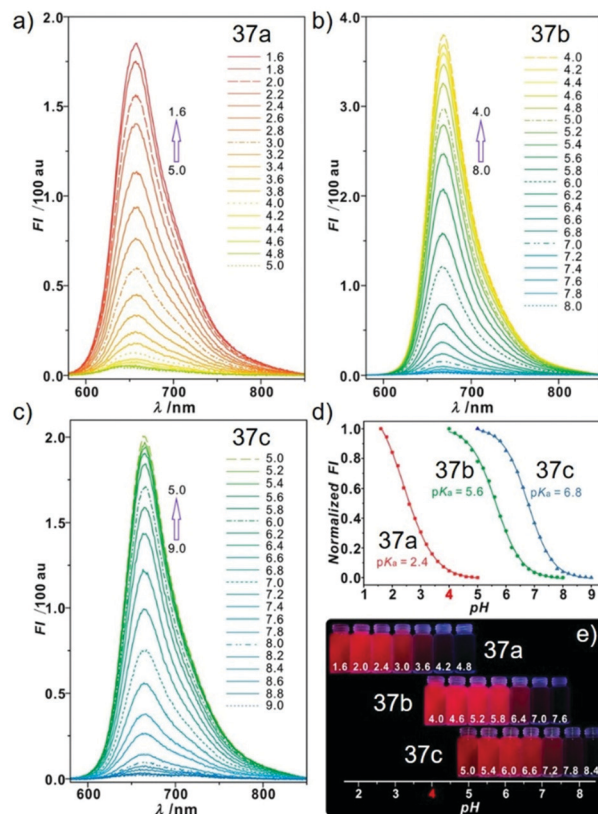
Fig. 56 pH activable emission properties of probes 37a–c (10 \mu M, \lambda_{ex} = 570 nm) in disodium hydrogen phosphate–citric acid buffers containing 10% DMSO: (a) probe 37a ; (b) probe 37b ; (c) probe 37c ; (d) normalized fluorescence intensities of probes 37a–c at different pH values at (a) 657 nm, (b) 668 nm, and (c) 663 nm; (e) photograph of pH-dependent red emissions under a 365 nm lamp in a darkroom. Copyright 2015 American Chemical Society.
