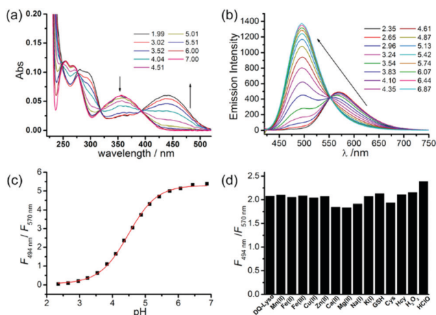
Fig. 44 (a) Absorption spectra of probe 29 (5 \mu\text{M} ). (b) Fluorescence spectra of probe 29 (2 \mu\text{M} ) in \text{Na}_2\text{HPO}_4 -citrate buffer (10 mM \text{Na}_2\text{HPO}_4 and 10 mM citric acid) at various pH values. (c) Ratio ( F_{494\text{nm}}/F_{570\text{nm}} ) changes as a function of the pH values. (d) Emission spectra of probe 29 (2 \mu\text{M} ) in the presence of various metal ions (100 \mu\text{M} \text{Mn}^{2+} , \text{Fe}^{3+} , \text{Fe}^{2+} , \text{Cu}^{2+} , \text{Zn}^{2+} , and 1 mM \text{Mg}^{2+} , \text{Ca}^{2+} , \text{Na}^+ , and \text{K}^+ ), 5 mM thiols (GSH, Cys, Hcy), and 100 \mu\text{M} \text{H}_2\text{O}_2 and \text{NaClO} in \text{Na}_2\text{HPO}_4 -citrate buffer (pH = 4.2); \lambda_{\text{ex}} = 405 nm. Copyright 2013 American Chemical Society.
