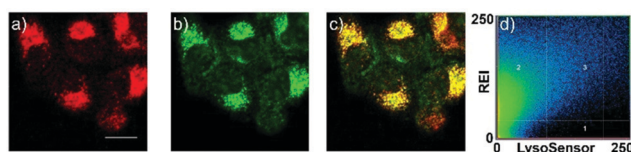
Fig. 16 Confocal fluorescence imaging of living HeLa cells co-stained with probe 12 (5 \mu M) and LysoSensor Green (1 \mu M) for 1 h. (a) Red emission from probe 12 ; (b) green emission from LysoSensor Green; (c) overlay of (a) and (b); areas of co-localization appeared in yellow; (d) the correlation of LysoSensor Green and probe 12 intensities. Copyright 2015 Elsevier.
