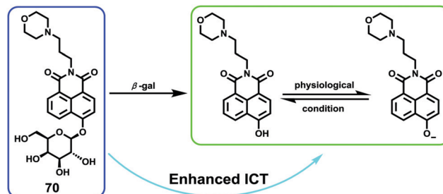
Scheme 56 Fluorescent probe 70 for \beta -gal.
