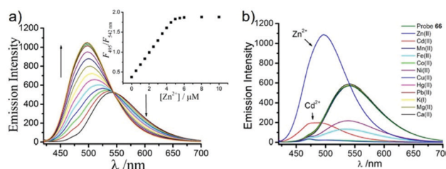
Fig. 110 (a) Fluorescence spectra of 5 \mu\text{M} 66 upon titration of Zn 2+ (0–10 \mu\text{M} ) in aqueous buffer (20 mM MES, 0.1 M NaCl, pH = 5.2), \lambda_{\text{ex}} = 405 nm. Inset: The emission ratio ( F_{495}/F_{542\text{nm}} ) changes as a function of Zn 2+ concentration. (b) Fluorescence spectra of 66 (5 \mu\text{M} ) in the presence of various metal ions (5 \mu\text{M} Mn 2+ , Fe 2+ , Co 2+ , Ni 2+ , Cu 2+ , Zn 2+ , Cd 2+ , and 1 mM Mg 2+ , Ca 2+ , and K + ) in MES buffer (pH = 5.2, \lambda_{\text{ex}} = 405 nm). Copyright 2012 American Chemical Society.
