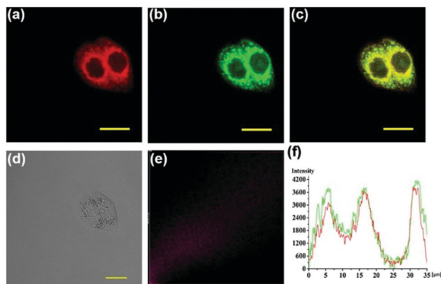
Fig. 96 Confocal images of HeLa cells treated with probe 60 (10 \mu M), \text{NaHSO}_3 (500 \mu M) and Lyso Tracker Red (75 nM). (a) Red channel (570–620 nm) for Lyso-Tracker Red under 561 nm excitation. (b) Green channel (500–550 nm) for probe 60 under 488 nm excitation. (c) The overlay image of red and green channels. (d) Bright-field of HeLa cells. (e) The intensity scatter plot of two channels. (f) Intensity profile of ROI across the cells in the red and green channels. Scale bar = 20 \mu m. Copyright 2018 Elsevier.
