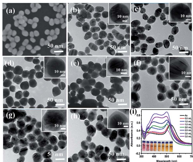
Fig. 2 (a) SEM image of Au NPs and (b–h) TEM images of the Au@Ag core-shell NPs synthesized under adding \text{AgNO}_3 in amounts from 0.50 to 3.50 mL at a gradient of 0.50 mL, respectively. The inset HRTEM images present the thickness of Ag shell from 1.0 to 10.0 nm; (i) the absorption spectra of Au NPs and Au@Ag core-shell NPs with the increase in the amount of \text{AgNO}_3 from 0.50 to 3.50 mL, the inset shows the colour of the solutions at different dosages of \text{AgNO}_3 solution.
