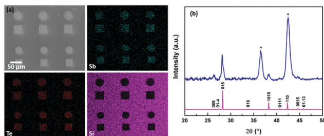
Fig. 1 (a) SEM image with EDX mapping and (b) grazing incidence XRD pattern from \text{Sb}_2\text{Te}_3 selectively deposited from [\text{SbCl}_3(\text{Te}^n\text{Bu}_2)_3] into 30 \mu\text{m} TiN holes and an indexed bulk pattern of \text{Sb}_2\text{Te}_3 . 42 The TiN substrate peaks are marked by *.
