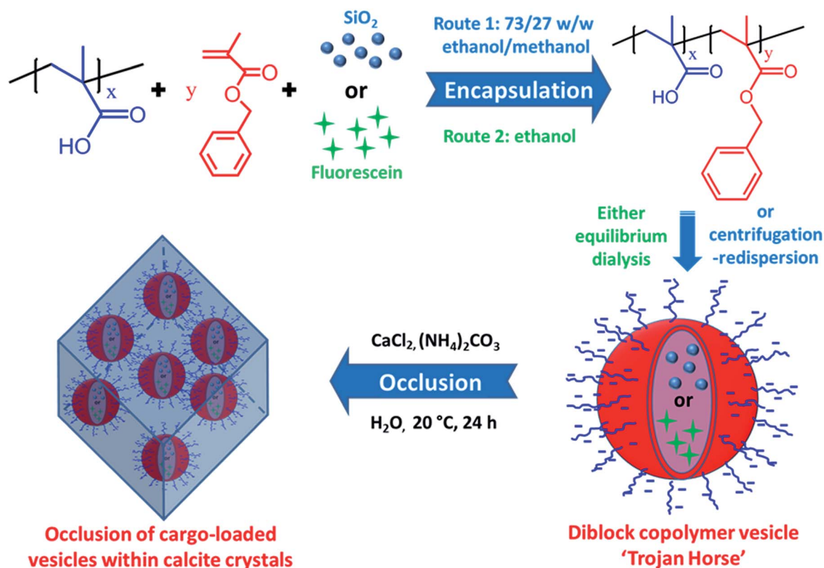
Scheme 1 Synthesis of poly(methacrylic acid) _x -poly(benzyl methacrylate) _y (PMAA _x -PBzMA _y ) vesicles at 20% w/w solids in the presence of either silica nanoparticles (Route 1) or fluorescein (Route 2) via RAFT dispersion polymerization of BzMA at 70^\circ\text{C} for 24 h. Excess silica nanoparticles or fluorescein dye were removed via either centrifugation-redispersion cycles (for the silica nanoparticles) or equilibrium dialysis (for the fluorescein dye). Schematic cartoon showing the occlusion of either silica-loaded or fluorescein-loaded PMAA _x -PBzMA _y vesicles within calcite ( \text{CaCO}_3 ) crystals.
