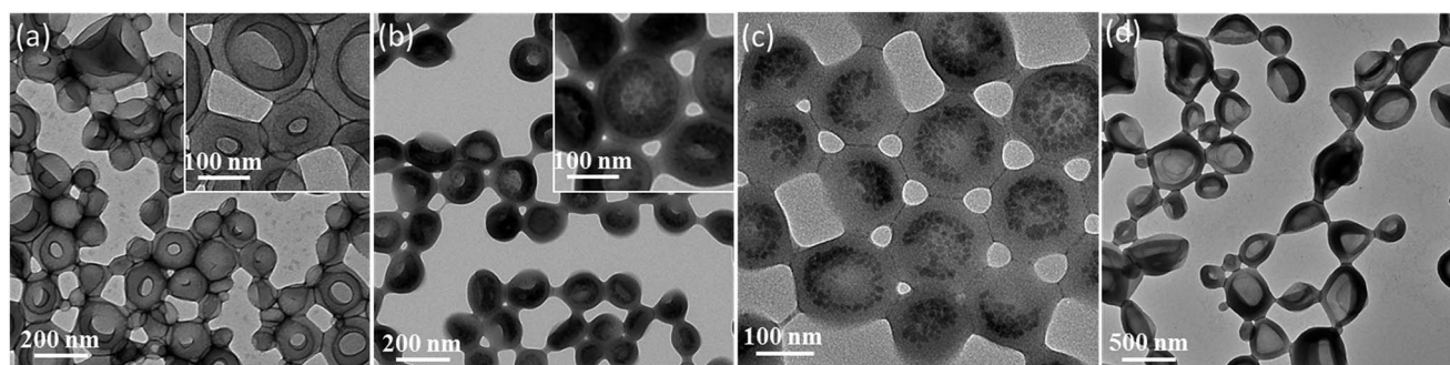
Fig. 1 Transmission electron microscopy (TEM) images recorded for: (a) stained PMAA _{69} -PBzMA _{200} vesicles prepared in the absence of any silica nanoparticles; (b) stained PMAA _{69} -PBzMA _{200} vesicles prepared in the presence of silica nanoparticles (after removing excess silica by multiple centrifugation-redispersion cycles); (c) unstained PMAA _{69} -PBzMA _{200} vesicles, clearly showing the encapsulation of silica within the vesicle lumen; (d) stained PMAA _{62} -PBzMA _{300} vesicles prepared in the presence of fluorescein dye (after removing excess dye via equilibrium dialysis). The vesicle aggregation observed in these TEM images is just a drying artefact.
