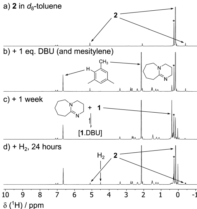
Fig. 4 The reversibility of the reaction between 1/[1]_2 , DBU and H_2 can be shown explicitly by a series of ^1H NMR spectra depicting: (a) a solution of 2 (0.03 mmol) in d_8 -toluene (0.5 mL) (b) the same solution with added DBU (0.03 mmol, 1 equivalent) and mesitylene (2%) as an internal standard; (c) after degassing three times over the course of one week, showing the formation of 1 \cdot DBU \leftrightarrow 1 \leftrightarrow [1]_2 ; (d) reformation of 2 after the addition of H_2 (4 bar). *Small amount of silicone grease from the independent synthesis of 2 .
