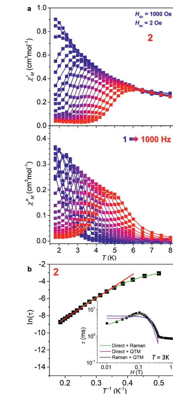
Fig. 4 (a) The in-phase ( \chi' ) and out-of-phase ( \chi'' ) components of the ac susceptibilities as a function of T of 2 in 1000 Oe dc field at different time frequencies (1–1000 Hz). (b) Natural logarithm of the relaxation time \ln \tau as a function of the inverse temperature T^{-1} . The straight red line is a fit of the 12 points at highest temperatures to the Arrhenius law \ln \tau = \ln \tau_0 + U_{\text{eff}}/k_B T . The curved green line is the best fit to the sum of the direct and Raman processes (see ESI†). Inset: field dependence of the magnetic relaxation times at 3 K for 2 and its approximation by the different models assuming two magnetic relaxation mechanisms, where only the sum of the direct and Raman processes gives a good fit.
