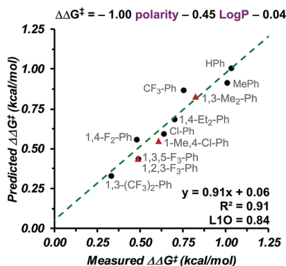
Fig. 3 Multidimensional correlation analysis showing the dependence of the reaction enantioselectivity on \log P and polarity of the aromatic solvent. The dataset includes 8 data points (black) and 3 external validations (red).
