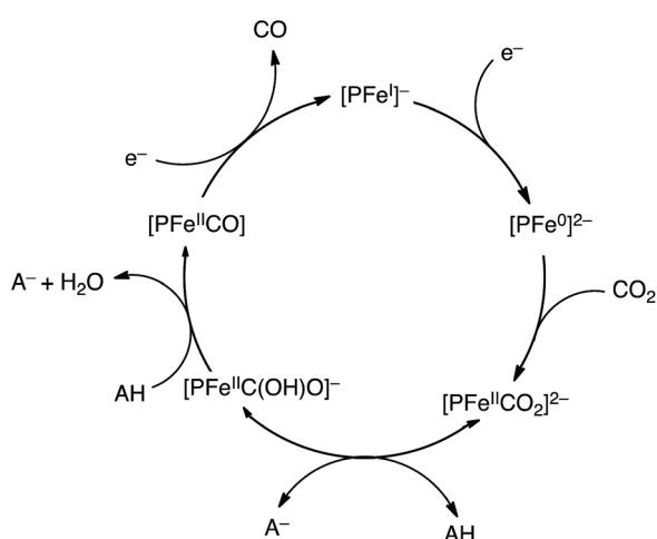
Scheme 3 Catalytic cycle for two-electron reduction of \text{CO}_2 to \text{CO} with an iron porphyrin ( [\text{PFe}]^- ). 84
