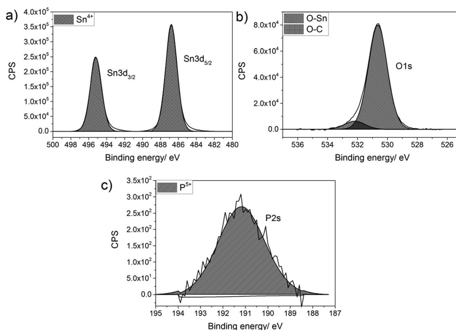
Fig. 1 Typical X-ray photoelectron spectra for (a) Sn 3d environment, (b) O 1s environment and (c) P 2s environment for P-doped SnO 2 films synthesised by AACVD at 550^\circ\text{C} .
